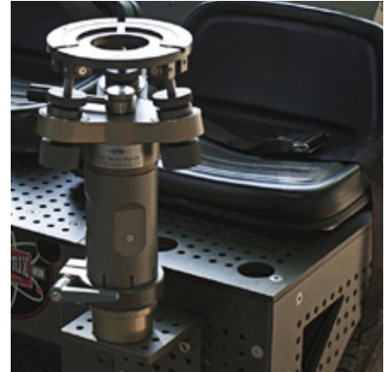
L-cheese plate with Euro-adaptor, Riser and Mitchell 3 Way Leveller
