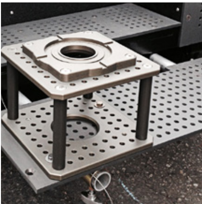
Mitchell plate with 10" cheese plate and connection rods
