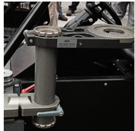
Euro-adaptor with GF-Swivel and GF-Combi-rig
