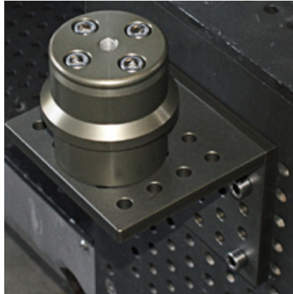
L-cheese plate with Euro-adaptor
